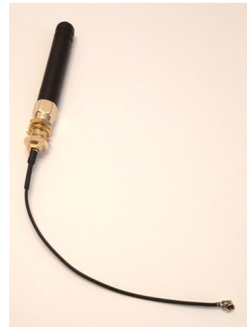
Figure 4. 868 MHz antenna.
